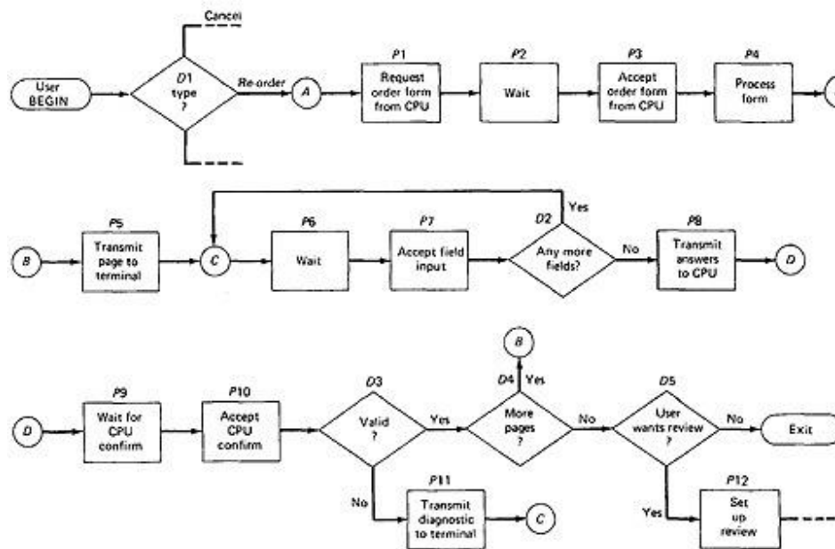
Figure 3.1: An Example of a Transaction Flow
