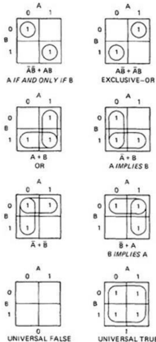
Figure 6.8: More Functions of Two Variables.
