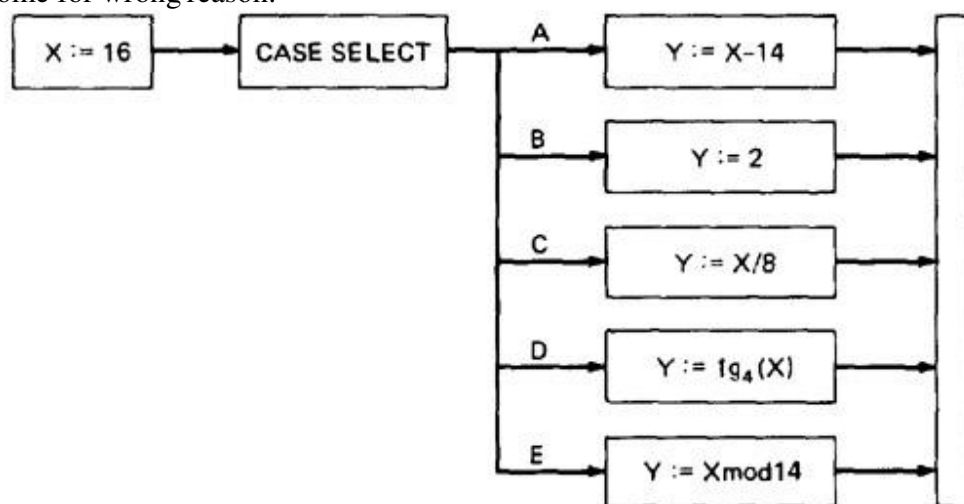
Figure 2.11: Coincidental Correctness
