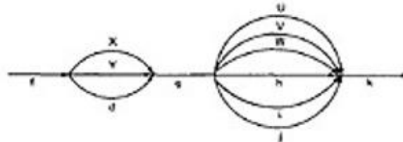
Figure 5.2: Examples of path sums.
