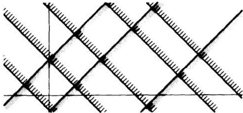
Figure 4.5: Tilted Boundaries.
