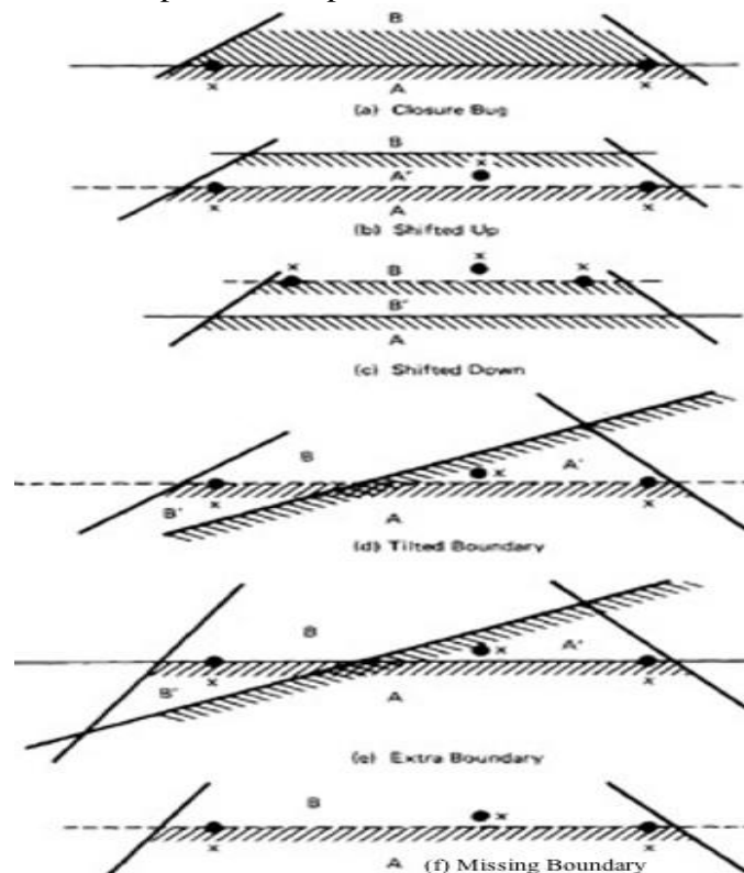
Figure 4.15: Two Dimensional Domain Bugs.
