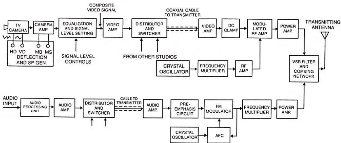
Fig. 23.34 Block Diagram of a Monochrome Transmitter
